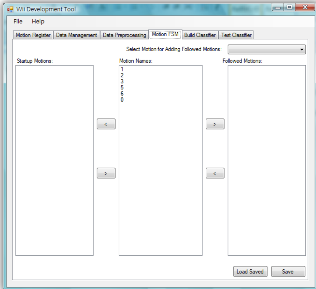
Fig 6.8 The Motion FSM Module
