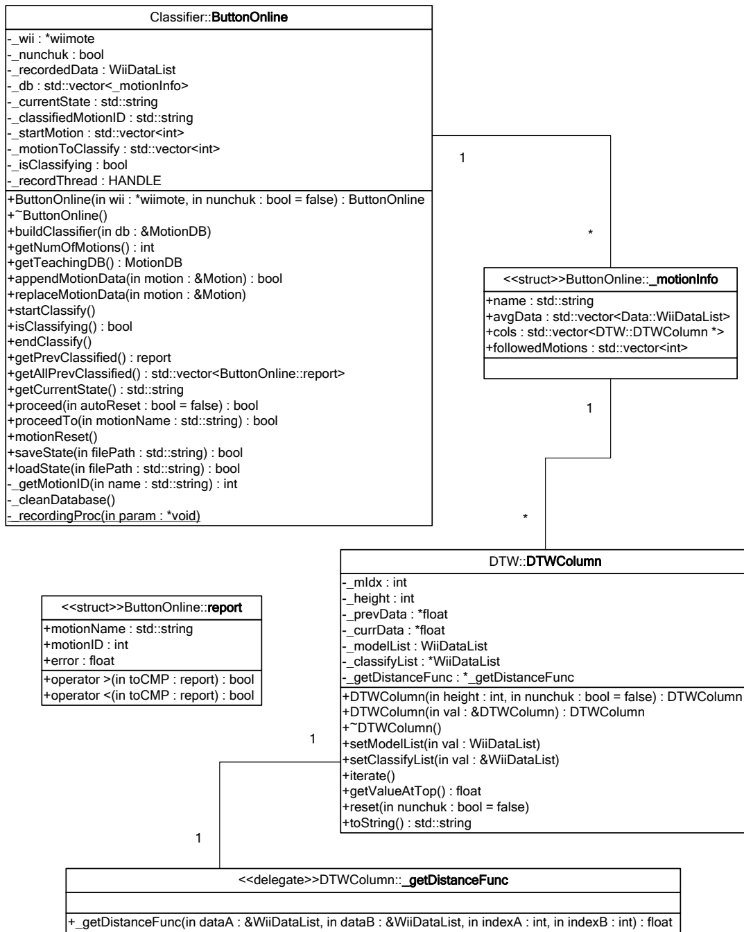
Fig 6.2 UML diagram for namespace WiiStyle::Classifier and WiiStyle::Classifier::DTW of Wii Style
