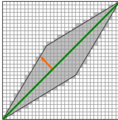
Fig. 3.14 A DWT grid with global constraints imposed.
