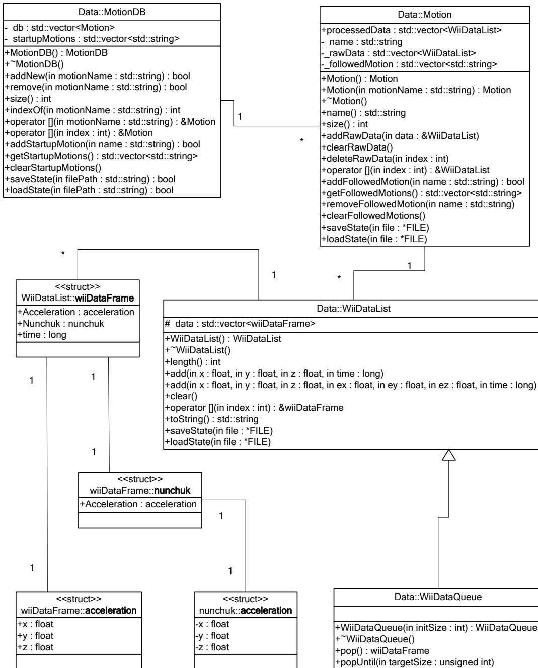
Fig 6.1 UML diagram for namespace WiiStyle::Data of Wii Style
