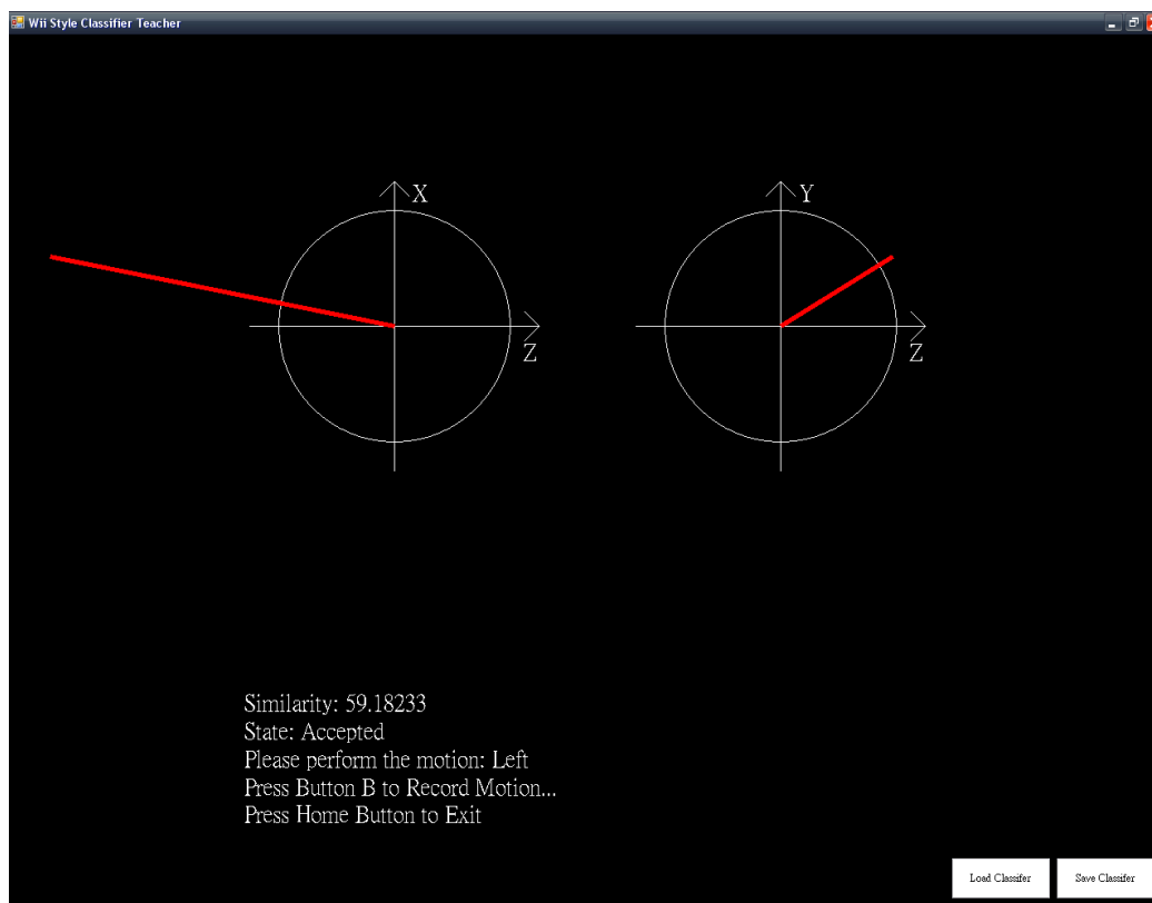
Fig. 7.4 Screenshot for Wii Style Classifier Teacher – the interface for teaching the classifier
