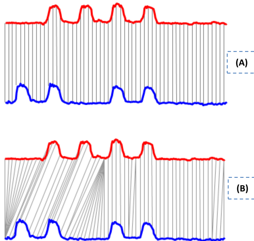
Fig. 3.15 Comparisons between Euclidean Distance algorithm (graph A) and Dynamic Time Warping (graph B) [11]
