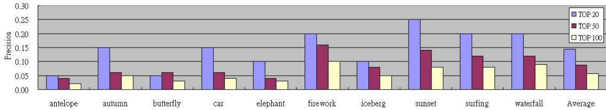
Figure 2: Experimental Results on 10 Testing Semantic Concepts
