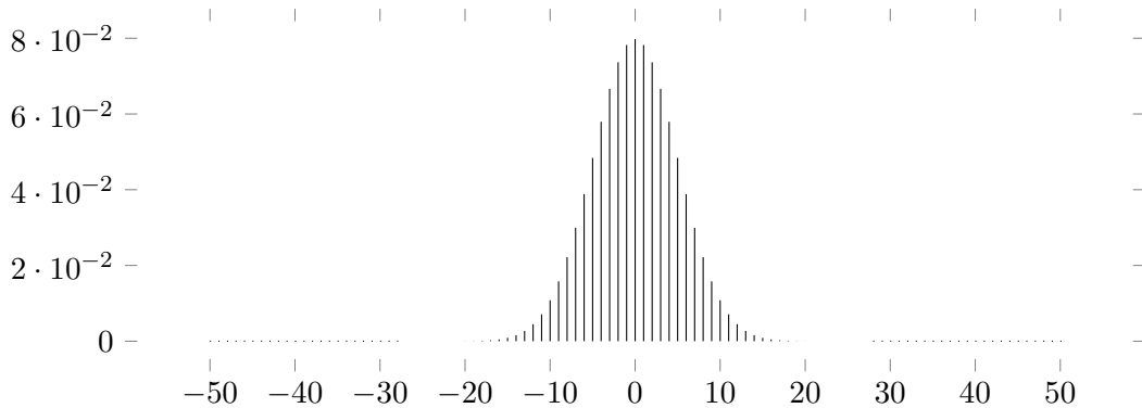
Figure 2: Discrete Gaussian noise over \mathbb{Z}_{101} with \sigma = 5 .
