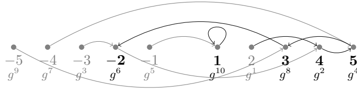
Figure 1: Powering in \mathbb{Z}_{11}^* . Arrows indicate squaring. The squares (in boldface) form the subgroup \mathbb{G} of quadratic residues modulo 11. Each has one positive and one negative square root.
