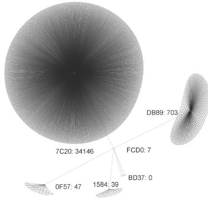
Fig. 14. Attack forensics of BD37 .
