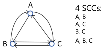
Fig. 12. A community structure with 3 nodes and 4 SCCs.
