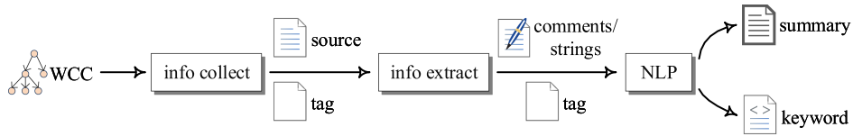
Fig. 16. Procedures of deanonymization.
