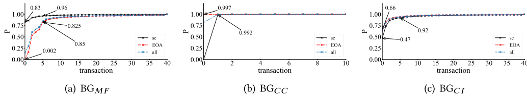
Fig. 2. Cumulative distribution of the number of transactions.
