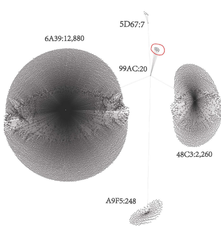
Fig. 17. The WCC rooted in 99AC.
