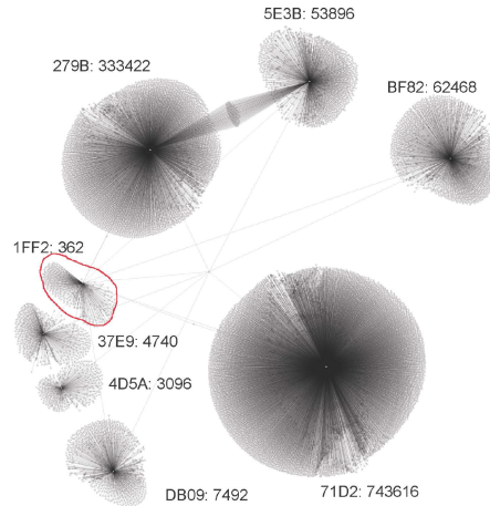
Fig. 18. The WCC rooted in 1Ff2.
