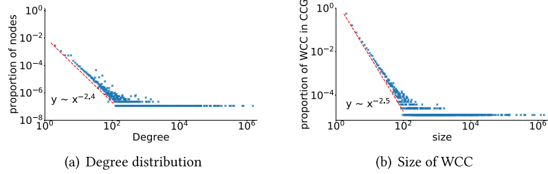
Fig. 9. Degree distribution and size of WCC of CCG.
