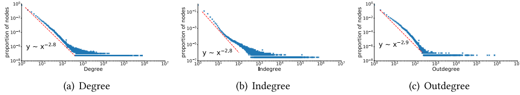
Fig. 11. Degree/Indegree/Outdegree distributions of CIG.
