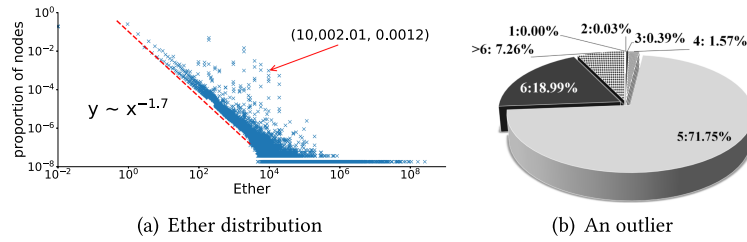
Fig. 6. Ether distribution and statistics of an outlier.
