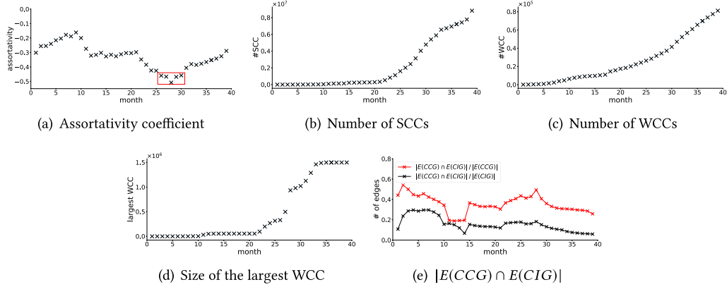
Fig. 10. Trend of CCG.
