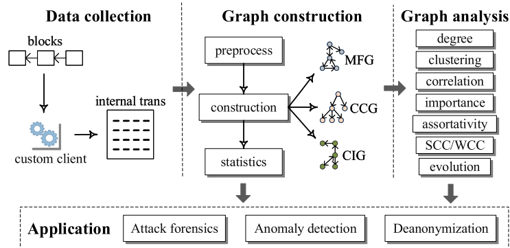
Fig. 1. An overview of our approach. Our approach consists of three phases, and we implement three applications based on graph analysis.
