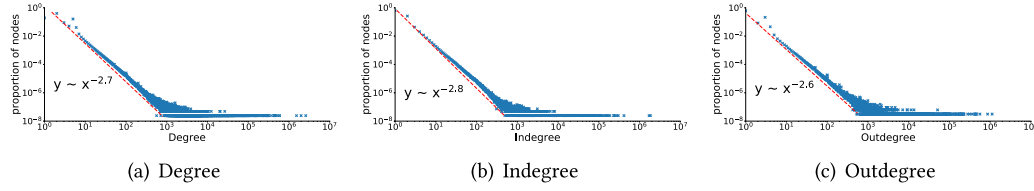
Fig. 5. Degree/Indegree/Outdegree distributions of MFG. They all follow power law.
