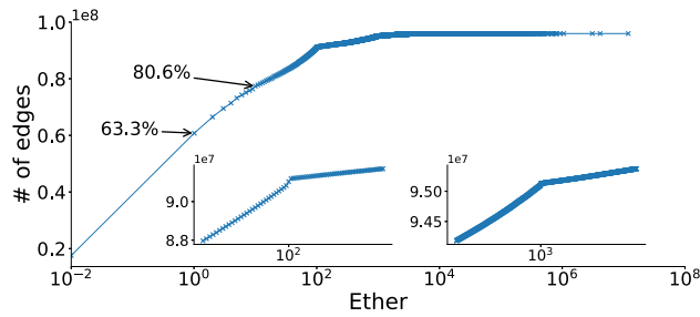
Fig. 7. Ether per transaction between two accounts.
