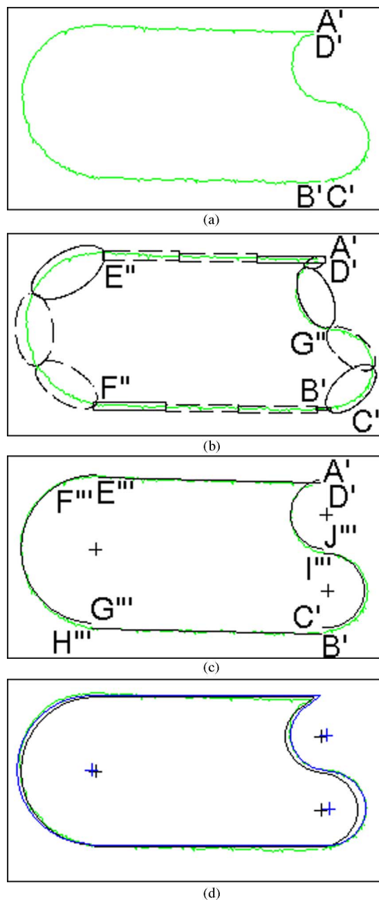
Fig. 1. Graphical primitives are extracted from a sketch. (a) A sketch with two strokes A'B' and C'D' . (b) Substrokes A'E'' , E''F'' , F''B' are extracted from stroke A'B' and C'G'' and G''D' are from C'D' . (c) Fitted results of substrokes are line segments A'E''' and H'''B' and arcs F'''G''' , C'I''' and J'''D' . (d) Refined graphical primitives are label in black, and ground-truth ones manually extracted in blue. (Color version available online at http://ieeexplore.ieee.org .)
