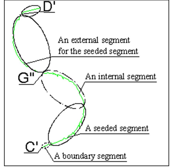
Fig. 2. Four categories of segments are for the substroke C'G'' . (Color version available online at http://ieeexplore.ieee.org .)
