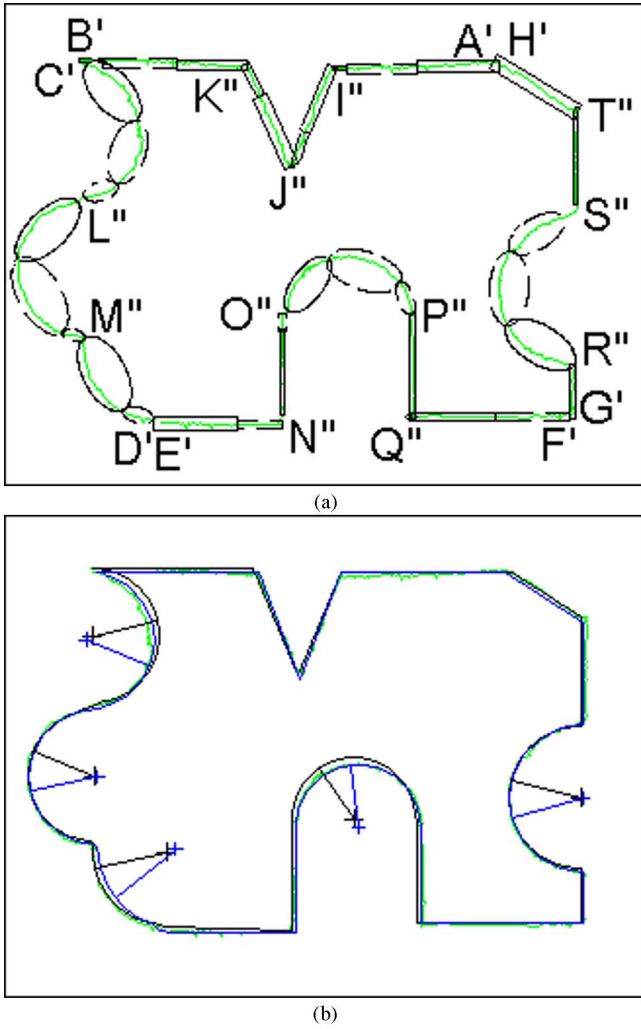
Fig. 4. Graphical primitives extracted from a sketch with part shape. (a) A sketch with four strokes A'B', C'D', E'F', G'H'. Substrokes A'I'', I'J'', J''K'', K''B' are extracted from stroke A'B', C'L'', L''M'', M''D' from C'D', E'N'', N''O'', O''P'', P''Q'', Q''F' from E'F', and G'R'', R''S'', S''T'', T''H' from G'H'. (b) Refined, ground-truth graphical primitives of the sketch are labeled in black and blue, respectively. (Color version available online at http://ieeexplore.ieee.org .)
