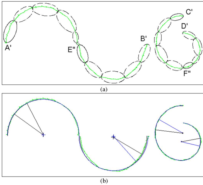
Fig. 6. Graphical primitives extracted from a sketch with externally and internally tangent arcs. (a) A sketch with two strokes, A'B' and C'D' . Substrokes A'E'' , E''B' are extracted from A'B' , C'F'' , F''D' from C'D' . (b) Refined, ground-truth graphical primitives of the sketch are labeled in black and blue, respectively. (Color version available online at http://ieeexplore.ieee.org .)
