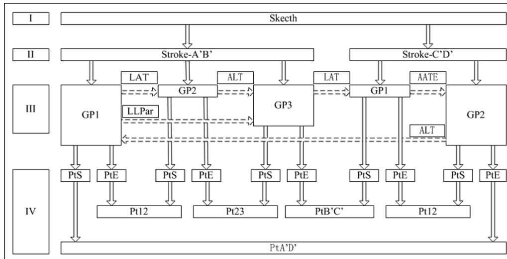
Fig. 3. Hierarchical network for the sketch shown in Fig. 1.
