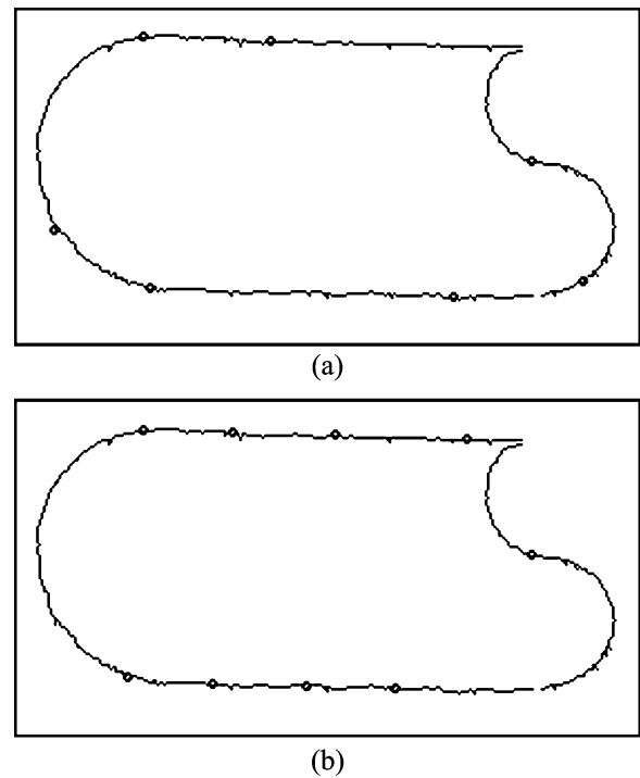
Fig. 7. Segmentation point detection results using two other approaches. (a) Segmentation points, marked by small circles, identified with the speed-threshold approach. (b) Segmentation points, marked by small circles, identified with the distance sign change approach.
