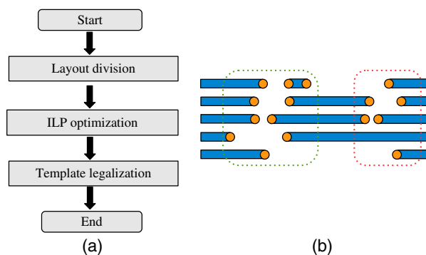
Fig. 4 (a) Overall flow of integer linear programming (ILP) speed-up method and (b) an example of layout division strategy.
