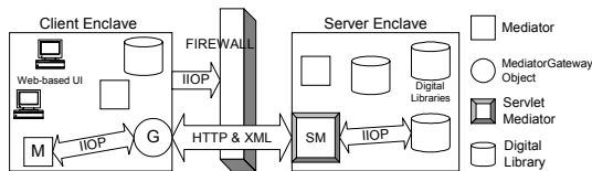
Figure 1. Using XML, HTTP & Servlet to support IIOP
