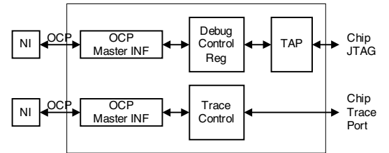
Figure 2: Block Diagram of Debug Agent
