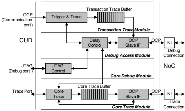
Figure 3: Debug Probe Block Diagram
