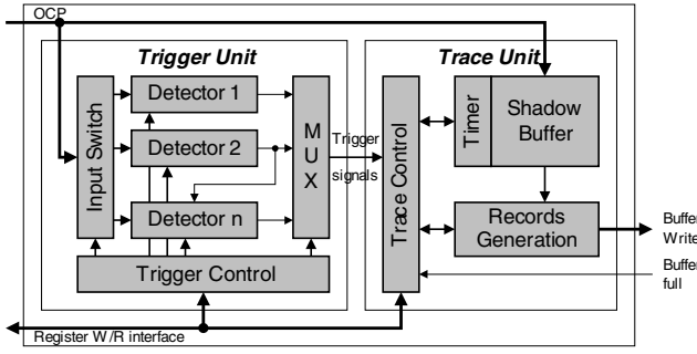
Figure 5: Transaction Trigger and Trace Unit
