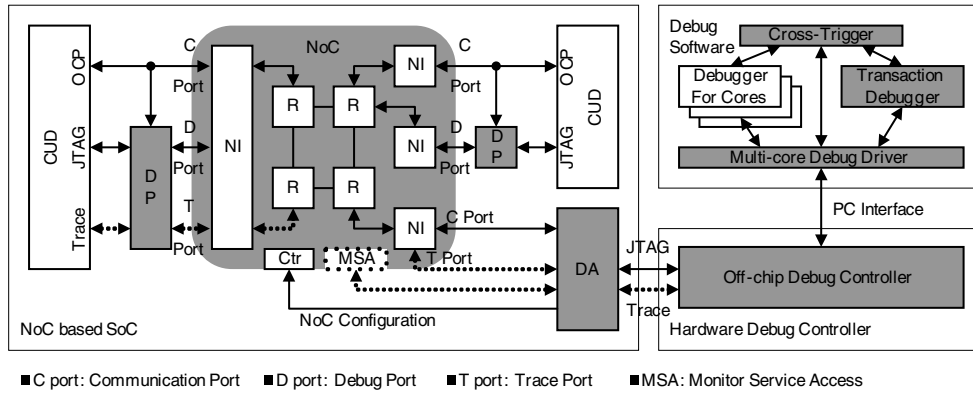
Figure 1: Debug Platform for NoC-based Systems
