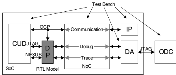
Figure 6: Simulation Environment
