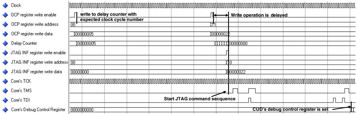
Figure 7: Simulation Waveform for the Delayed Write Operation
