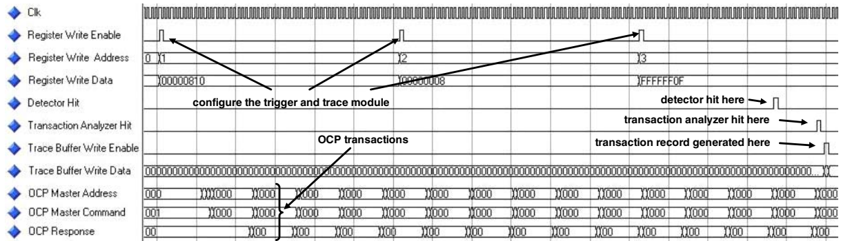
Figure 8: Simulation Waveform for the Transaction Trace Operation
