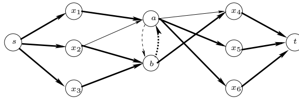
Figure 5: The flow network corresponding to the \text{SOFT\_SAME}^{var}(S_1, S_2) constraint
